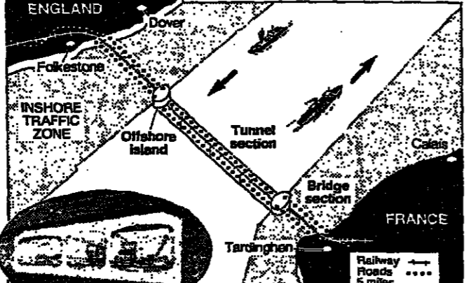
The Euroroute scheme. Inset: The railway flanked by road lanes in the tunnel section.
